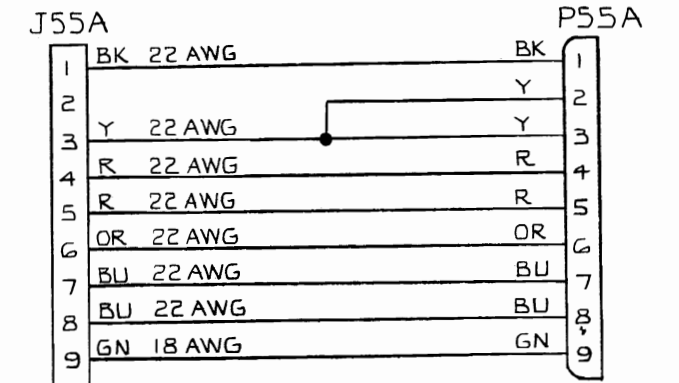
Coin Option Interconnect Wiring Diagram
