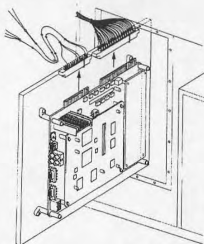
JAMMA standard cabinet, for example
