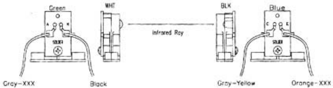
Photo Transistor Board (A-16909) Receiver 0.1-0.7V Unblocked 11-13V Blocked
