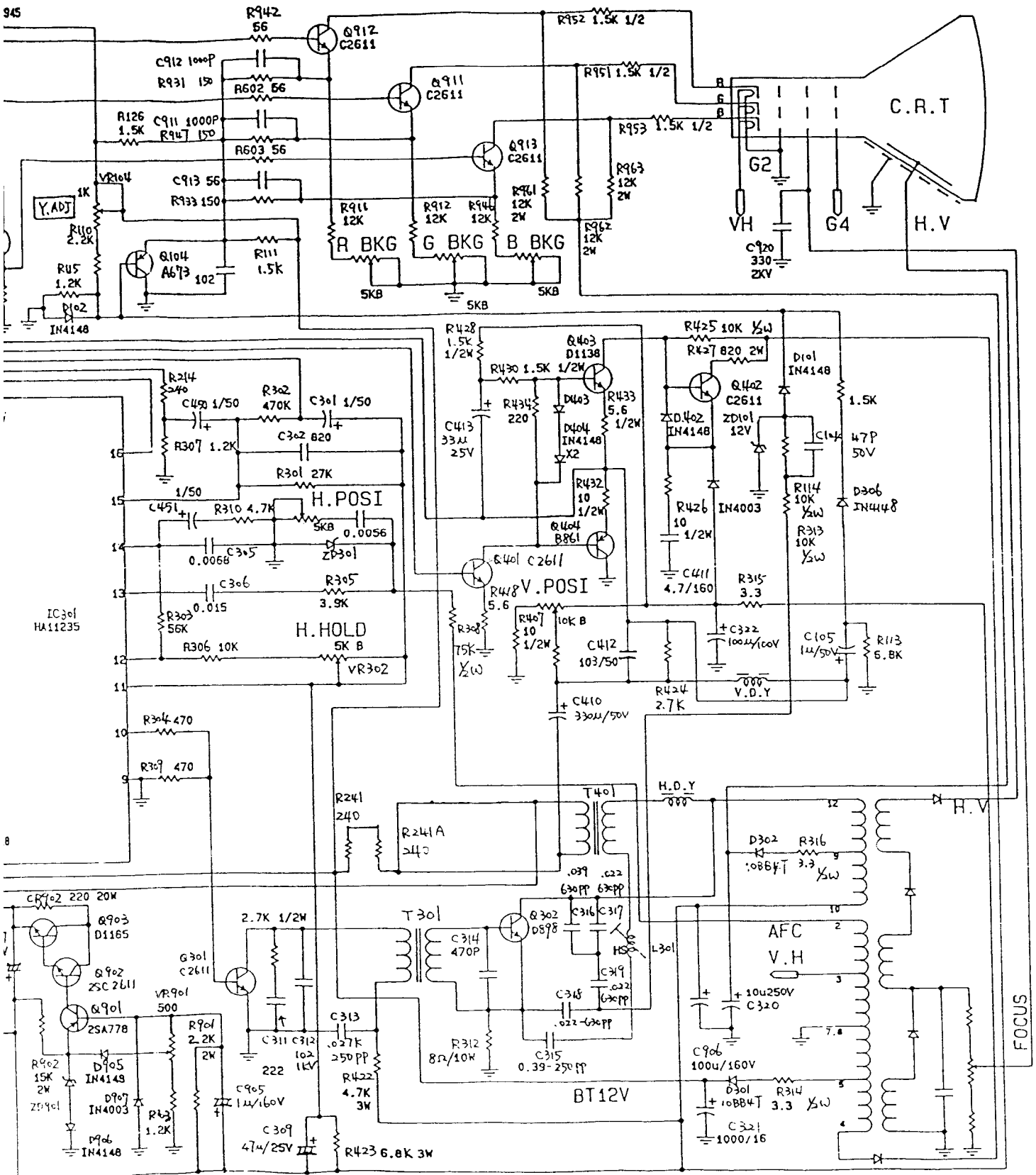
20" TV CHASSIS CIRCUIT DIAGRAM
