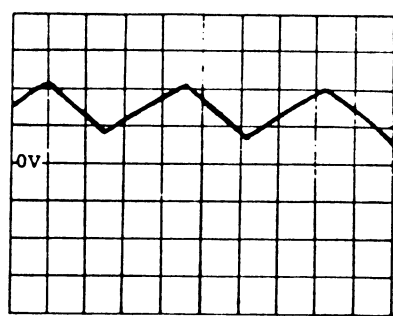
555 Pin 2 5V/DIV. 10uS
