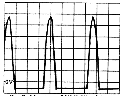
Q 3 Collector 50V/DIV. 10uS
