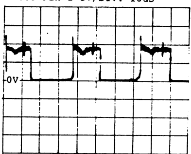
Q 1 Collector 5V/DIV. 10uS
