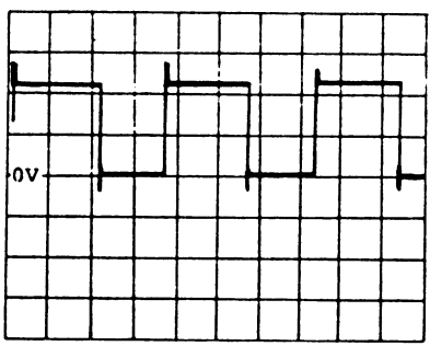
555 Pin 3 5V/DIV. 10uS
