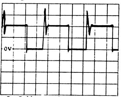
Q 1 Collector 20V/DIV. 10uS
